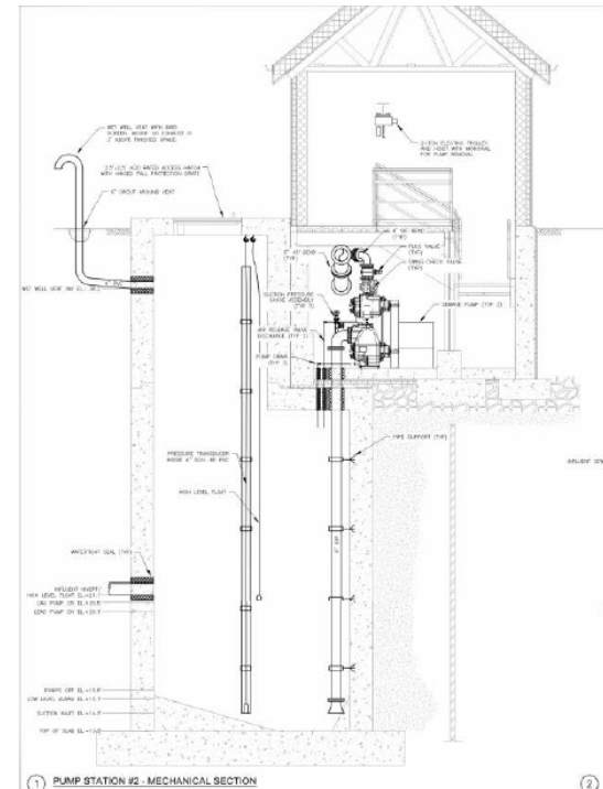
1 PUMP STATION #2 - MECHANICAL SECTION
